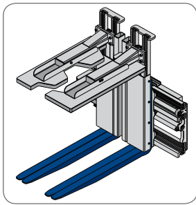
Single-Double with Load Hold-Down for double high stacks
