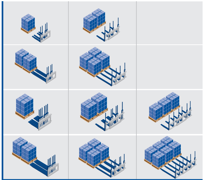
Single-Double Pallet Handler Model FDS • 1-2 Pallets
